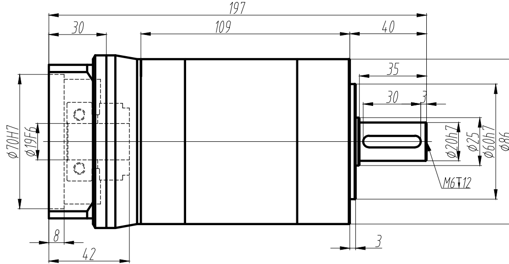
标准轴 Standard output shaft
